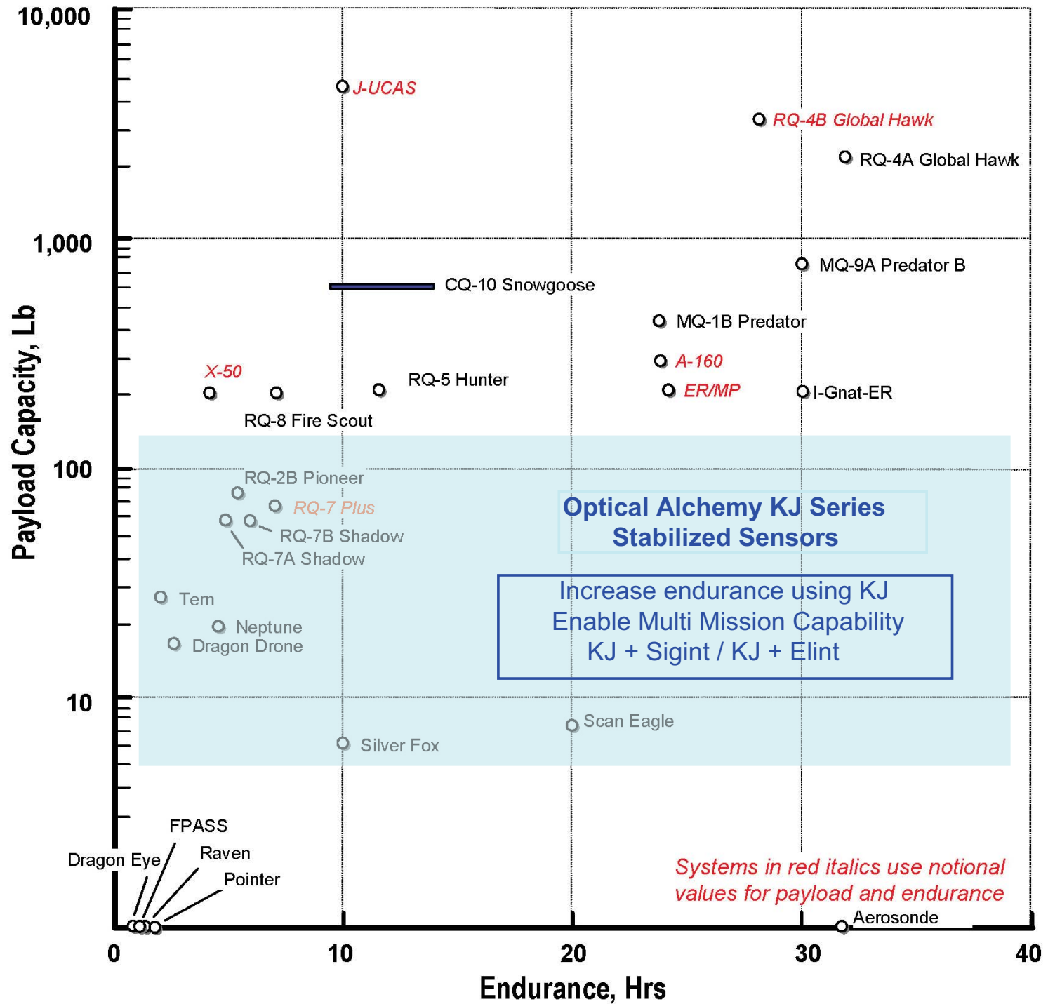
FIGURE 4.4-1. UA PAYLOAD CAPACITY VS. ENDURANCE.
